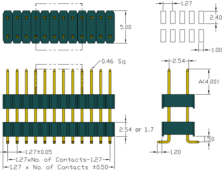
Recommended P.C.Board SMD Layout
